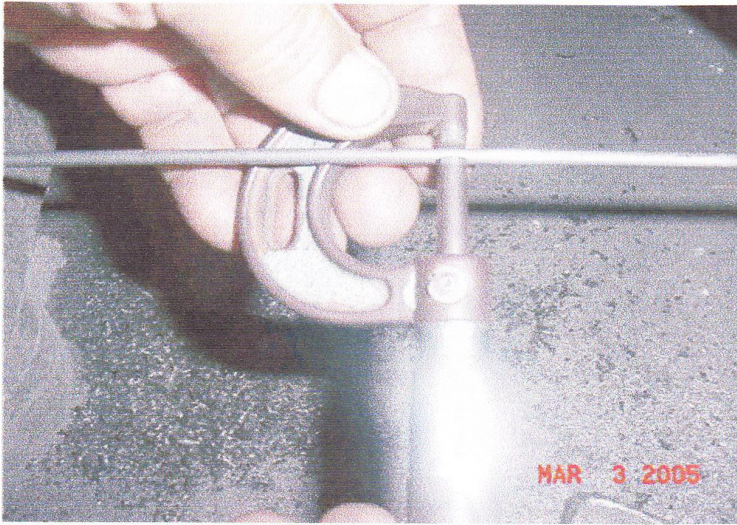
DIAMETER INSPECTION
